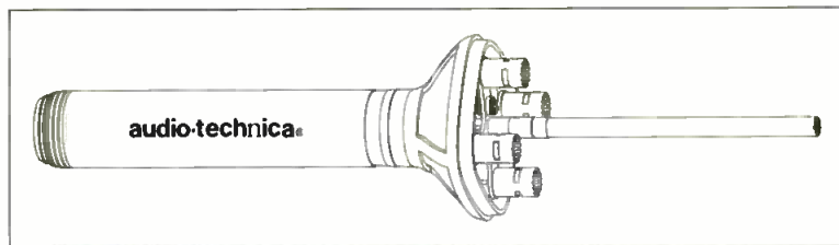
Beneath the grille, the Audio-Technica AT895 Adaptive-array Microphone houses five discrete microphone elements.
